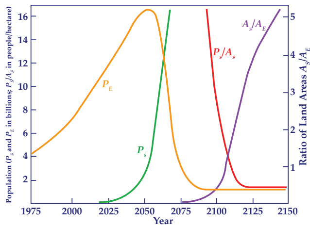
Figure 1 — A graph, technically realizable in my opinion, showing that most industry could be removed from the biosphere of the Earth within a century. The graph is based on a "worst-case" assumption: no reduction of the population growth rate either on earth or in the space communities. P_E is the population on earth, P_S the population in space, A_S/A_E the ratio of land area in space (all usable) to the total land area of Earth. Changes within wide limits in the assumed input numbers do not affect reaching a solution stable in P_E and P_S/A_S . The final stable value of P_E ( 1.2 \times 10^9 people) is equivalent to the 1910 value.
