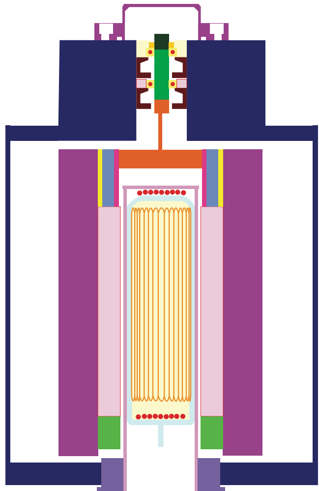
Figure 5 — Electromechanical Battery
