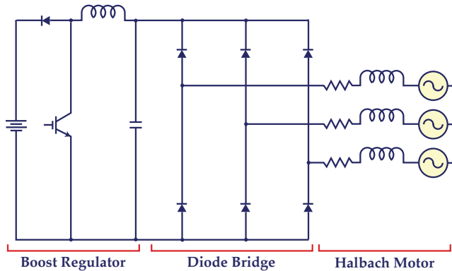
Figure 7 — Simplified Schematic of Energy Extraction Circuit
