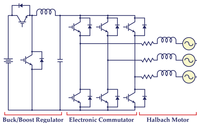
Figure 8 — Simplified Schematic of Electromechanical Battery
