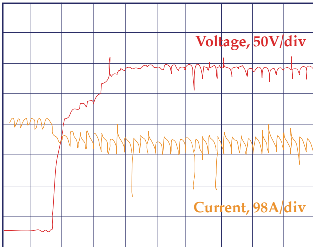
Figure 10 — Bridge Current and Voltage During Extraction
