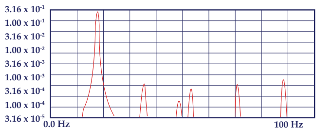
Figure 9b — Open Circuit Voltage Harmonics
