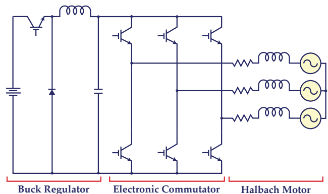
Figure 6 — Simplified Schematic of Spin-up Circuit
