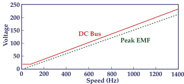
Figure 11 — Flywheel Speed versus DC Bus Voltage Graph
