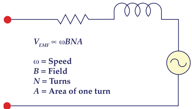
Figure 4 — Equivalent Circuit for Electric Machine, per Phase Basis
