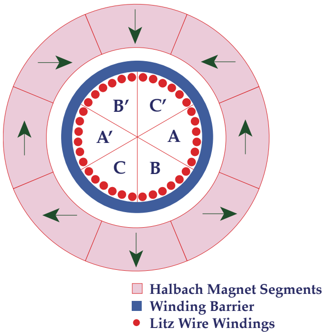
Figure 3 — Halbach Array with Three Phase Winding
