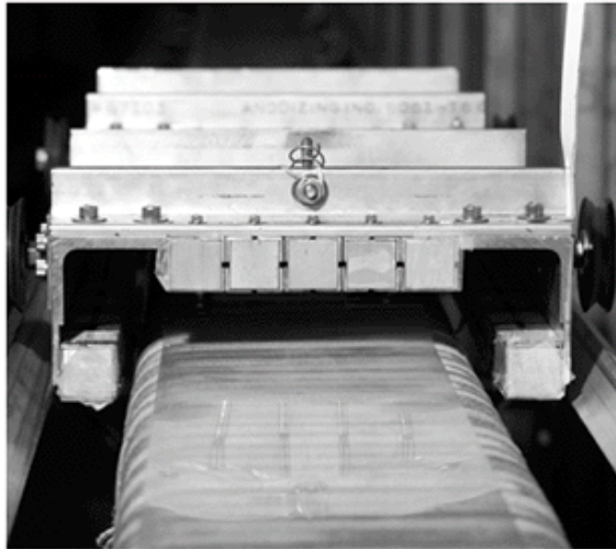
Figure 2. The test cart in motion levitated above the test track. The Halbach arrays can be seen beneath the cart and suspended from its sides. These arrays generate a magnetic field that induces, from the motion of the car, currents in the coils contained in the track, lifting and centering the cart above the track.
